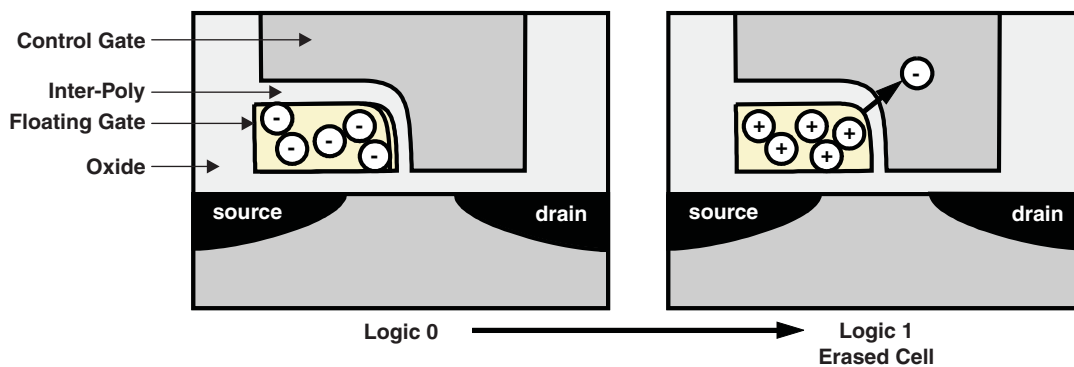
Figure 2. Erasure of Flash Memory Cell (Erased Cell Is on the Right)
