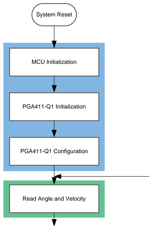
Figure 1. Software Flowchart
