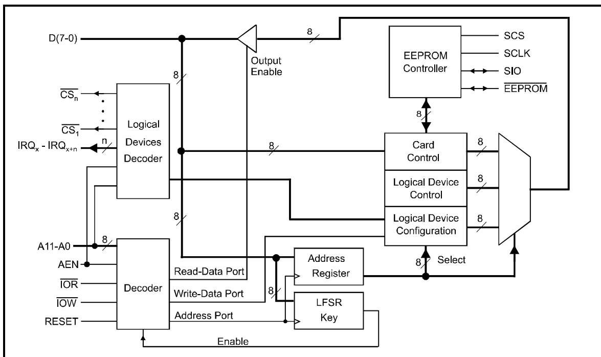
Figure 1: Block circuit diagram of a PnP logic circuit
