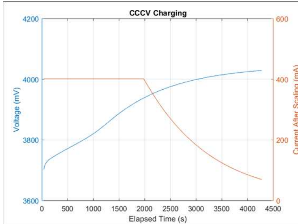
Figure 2. Charging Profile
