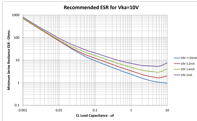
Figure 7. ESRs @ Vka=10V
