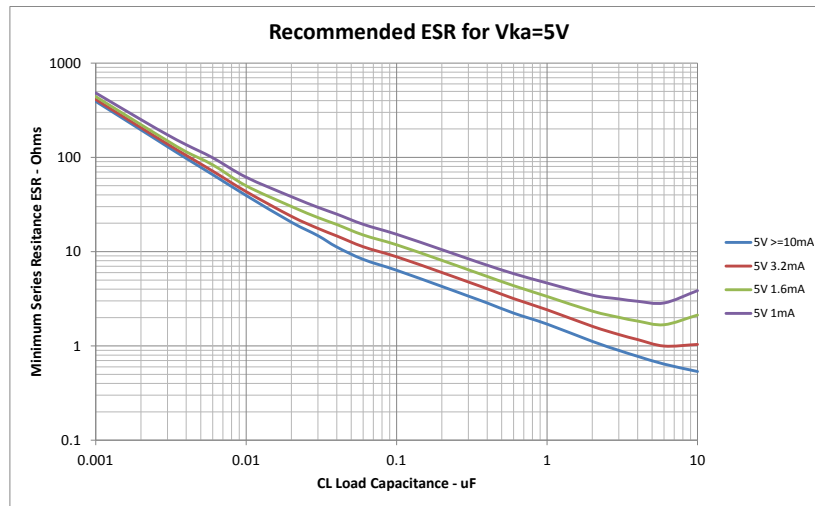
Figure 6. ESRs @ Vka=5V
