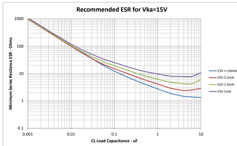
Figure 8. ESRs @ Vka=15V
