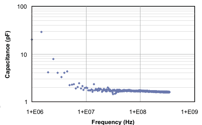
Figure 2. REF_IN Shunt Capacitance vs. Frequency
