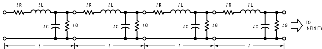
Figure 5. A Transmission Line Model Composed of Short, Series Connected Sections
