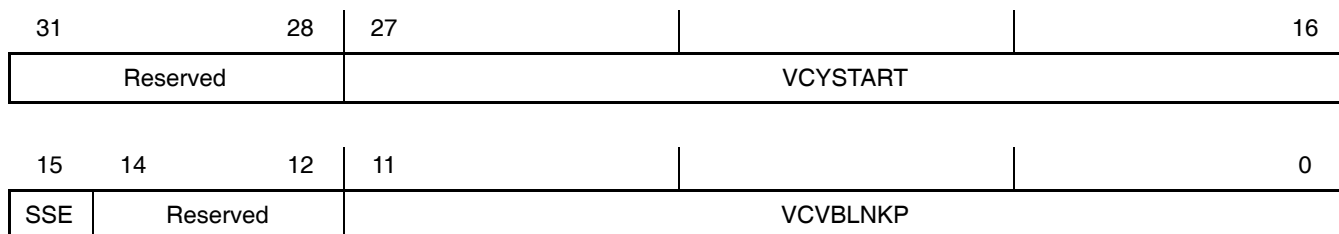
Figure 5. VCxSTRT1 Register
