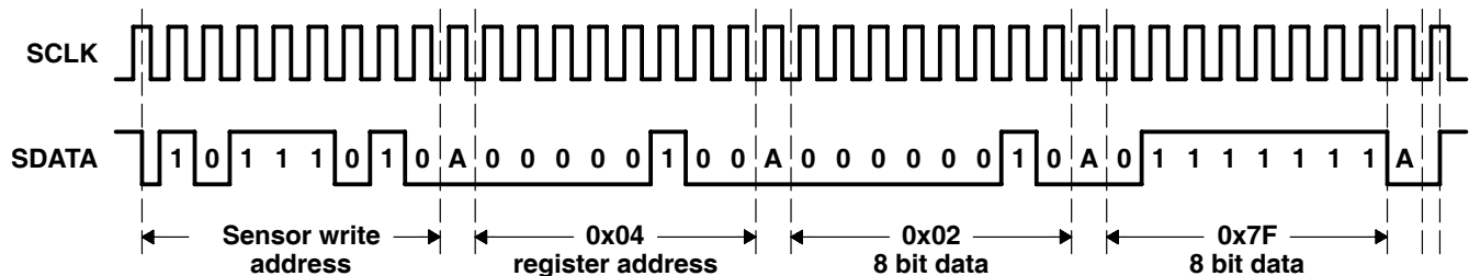
Figure 2. I 2 C Write to Column Size Register (0x04) with the Value 0x027F
