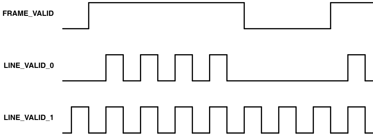
Figure 1. Non-Continuous and Continuous LINE_VALID Formats
