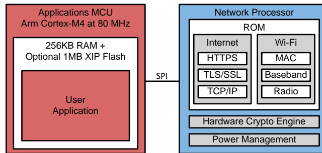
Figure 7. Separate Execution Environments
