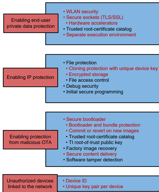
Figure 6. E-Lock Security Challenges and SimpleLink™ Wi-Fi Security Enablers
