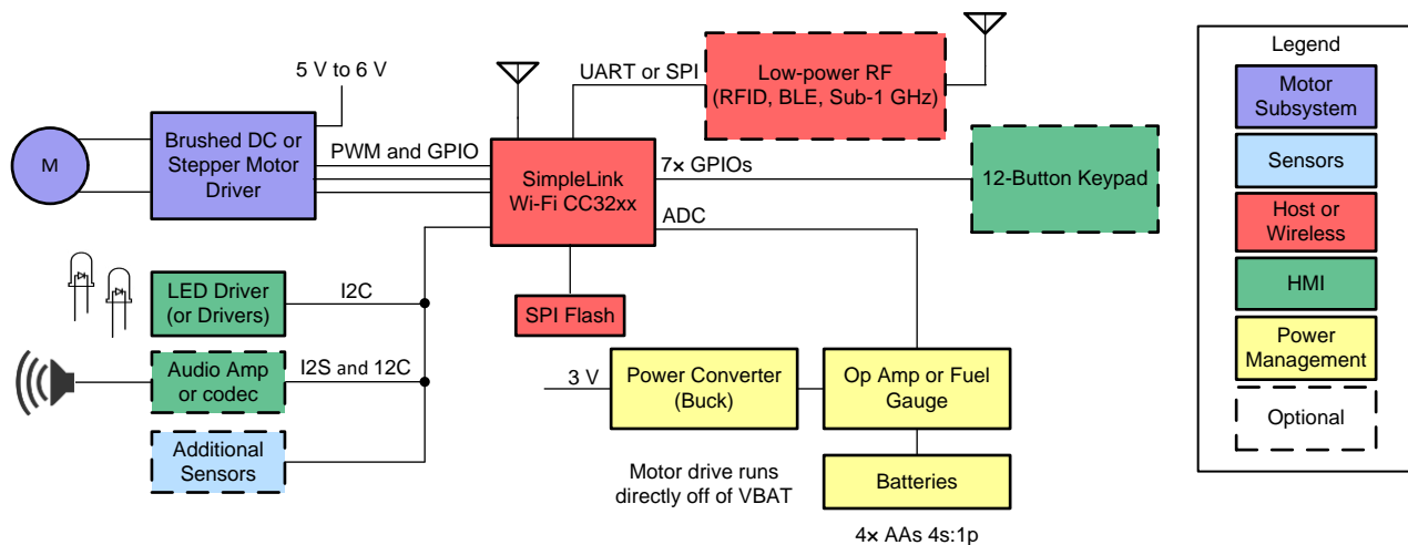
Figure 2. Example Wi-Fi Enabled E-Lock System Block Diagram
