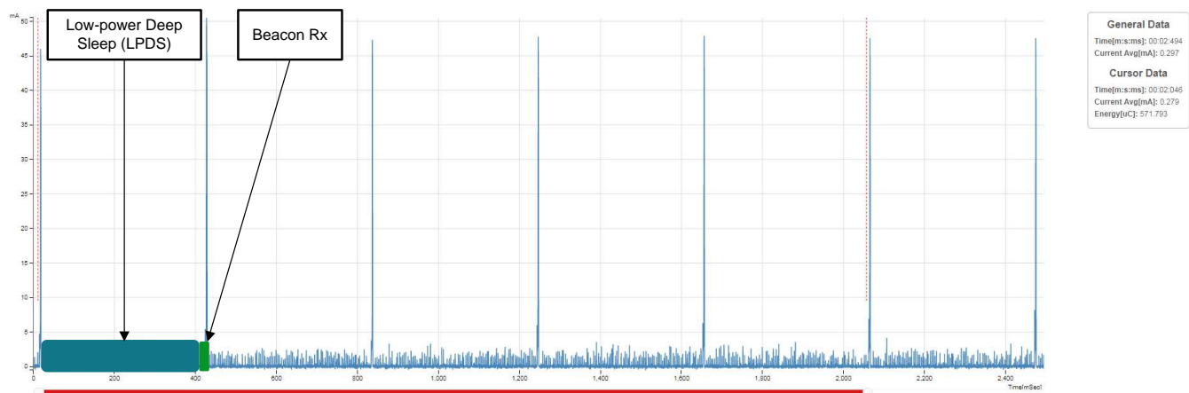
Figure 5. Always Connected Idle Current With LSI = 500 milliseconds
