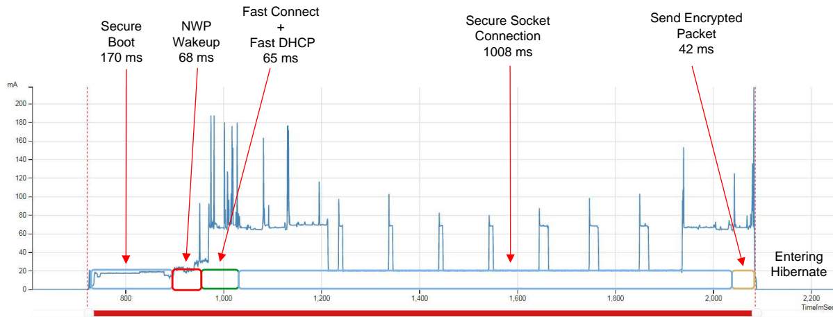
Figure 4. Power Consumption of CC3220S From Hibernate to TLS Connection to www.google.com
