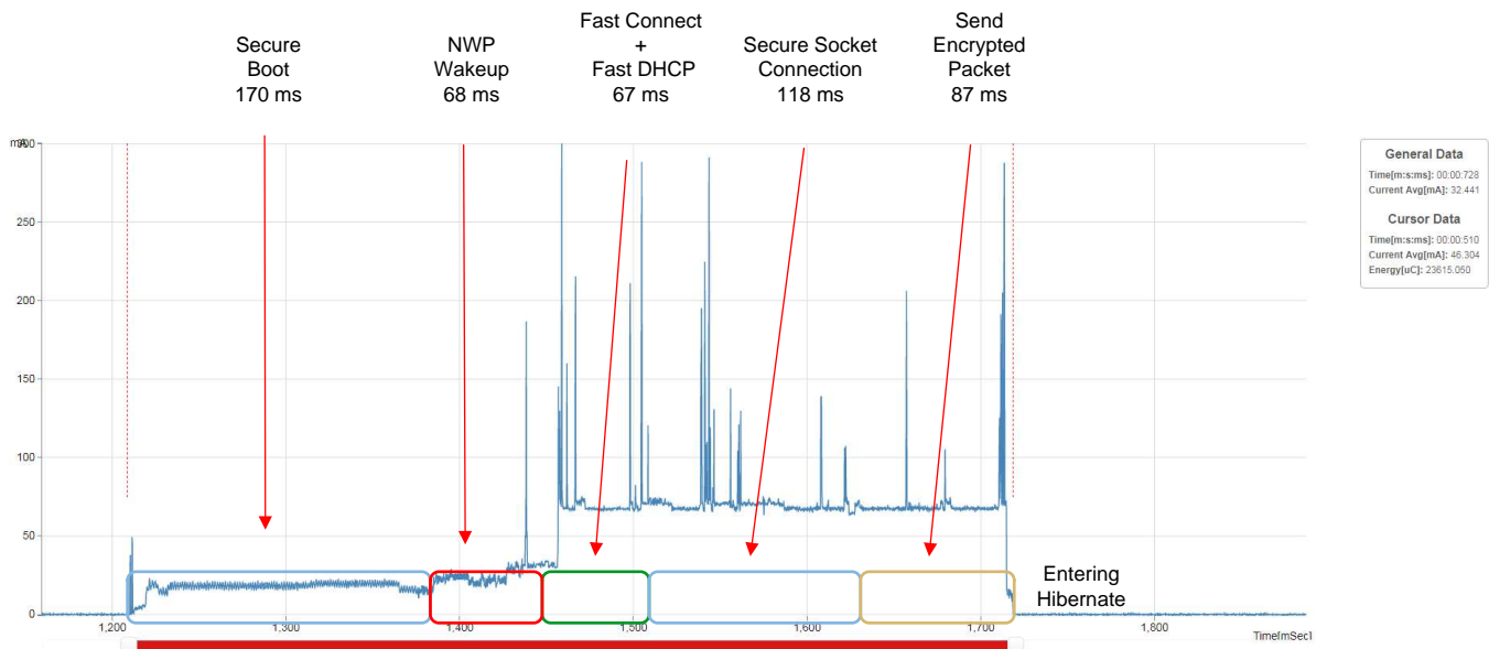
Figure 3. Power Consumption of CC3220S From Hibernate to TLS Connection to Local Server
