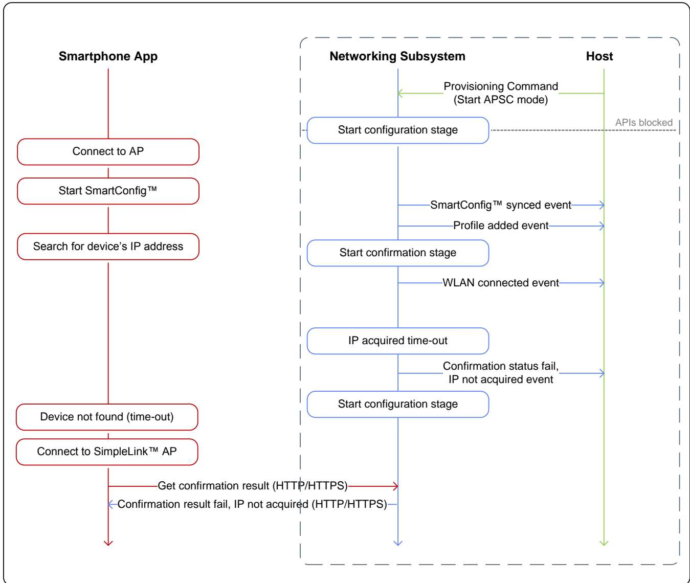
Figure 4. Unsuccessful SC Provisioning Example
