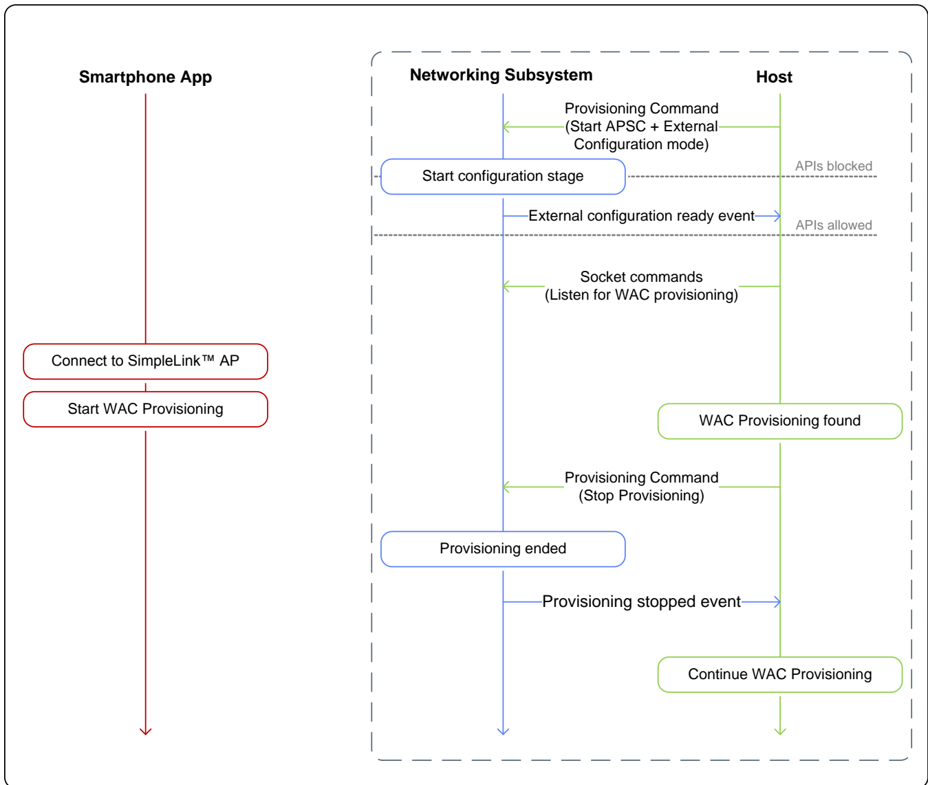
Figure 8. WAC Provisioning Example
