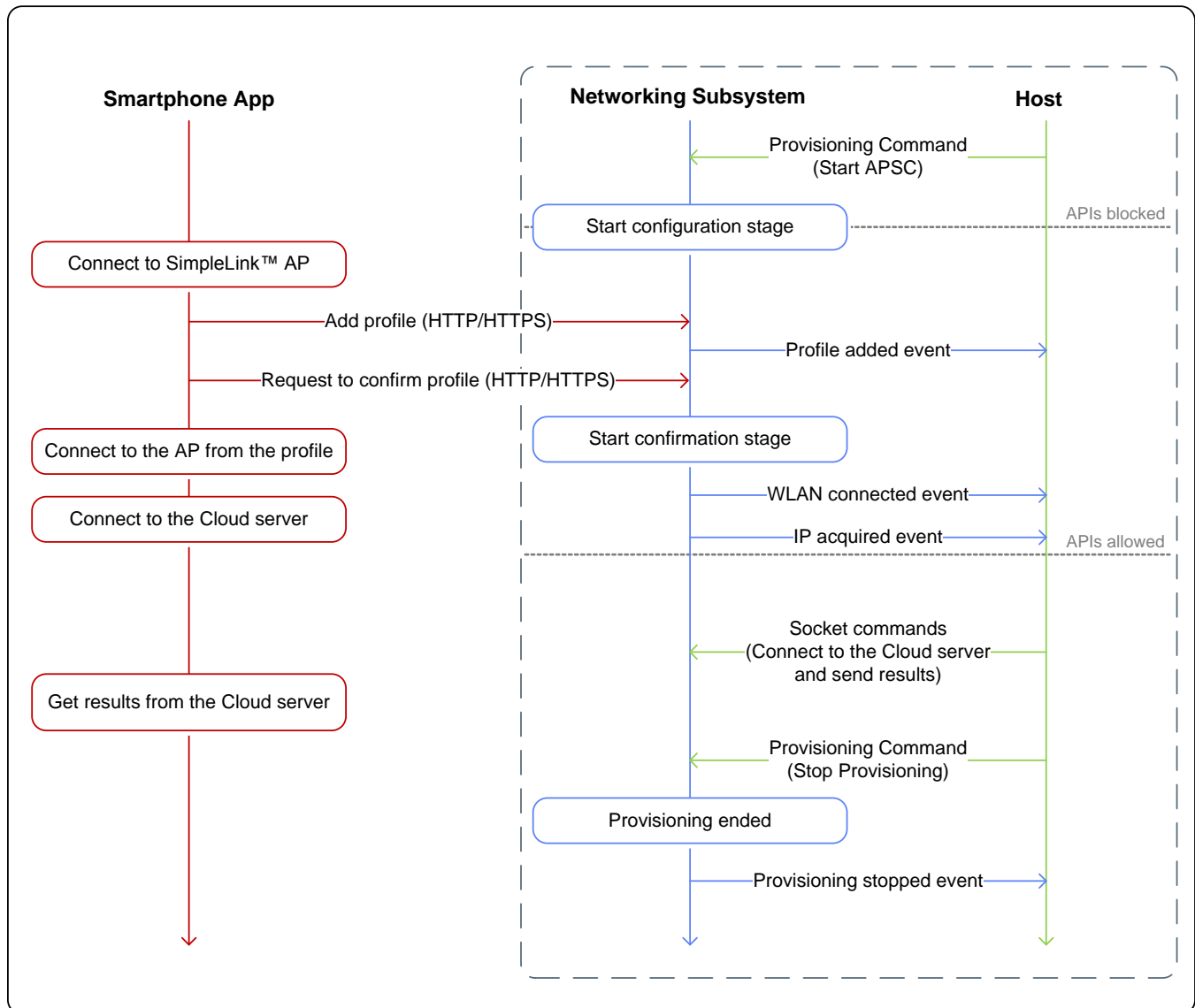
Figure 7. Successful AP Provisioning Cloud Example
