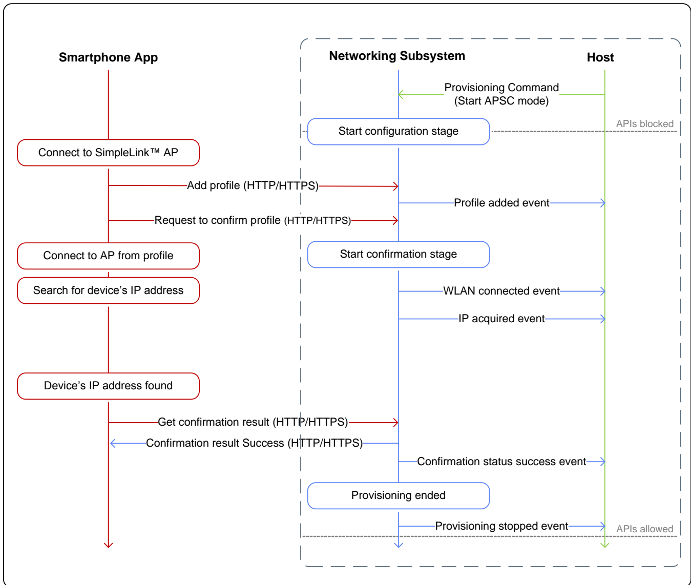
Figure 6. Successful AP Provisioning Example
