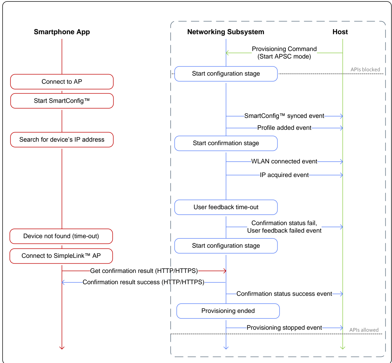
Figure 5. Successful SC Provisioning with AP Fallback Example
