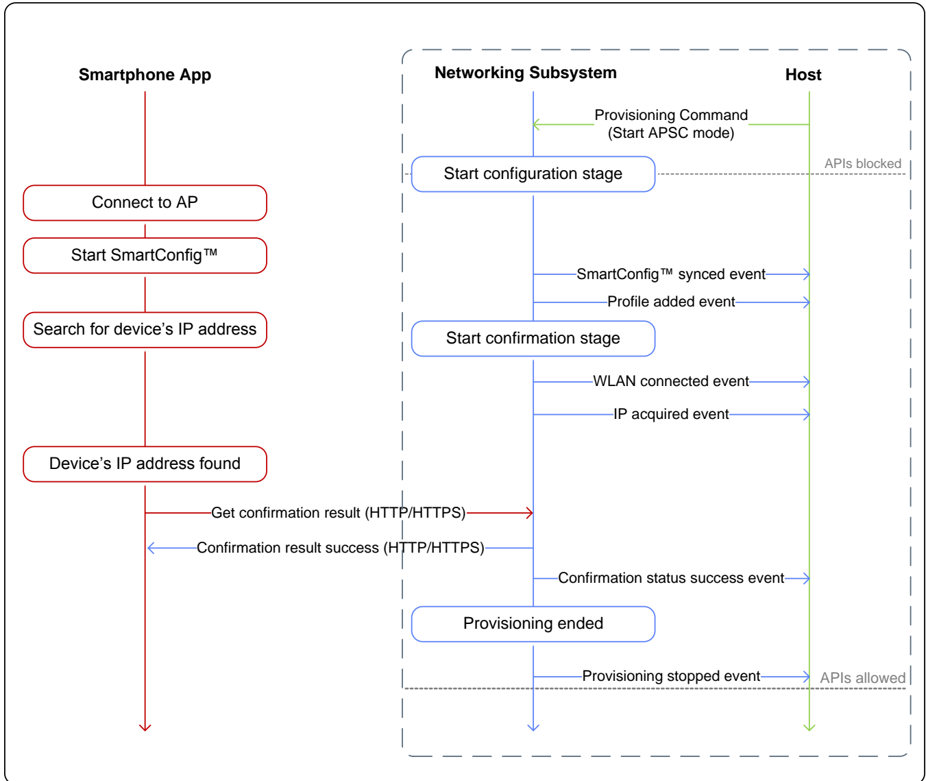
Figure 3. Successful SC Provisioning Example
