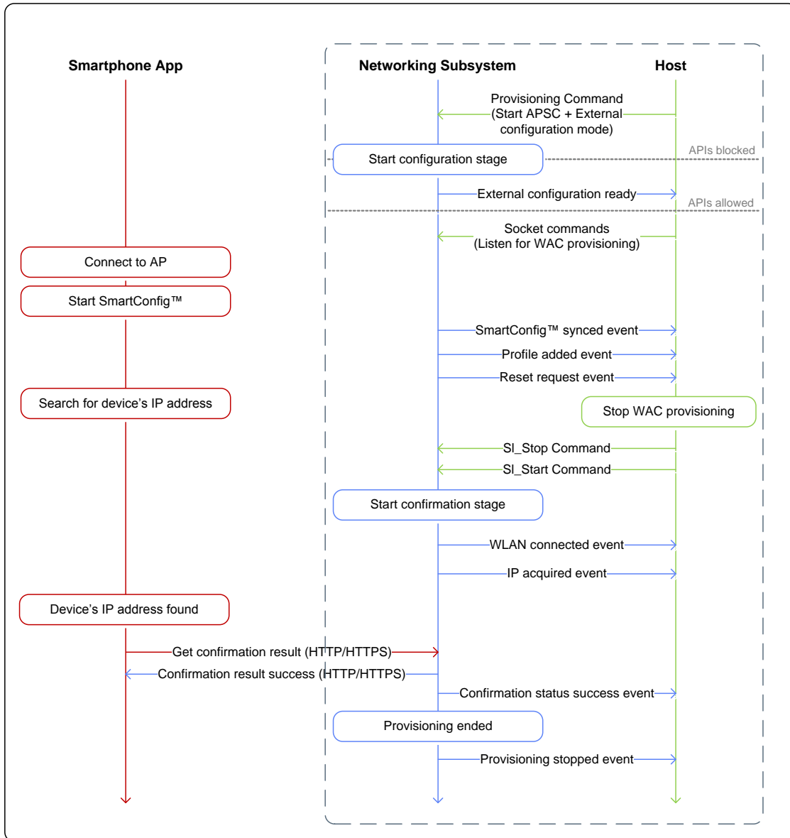
Figure 9. Successful SC Provisioning While External Configuration Enabled Example
