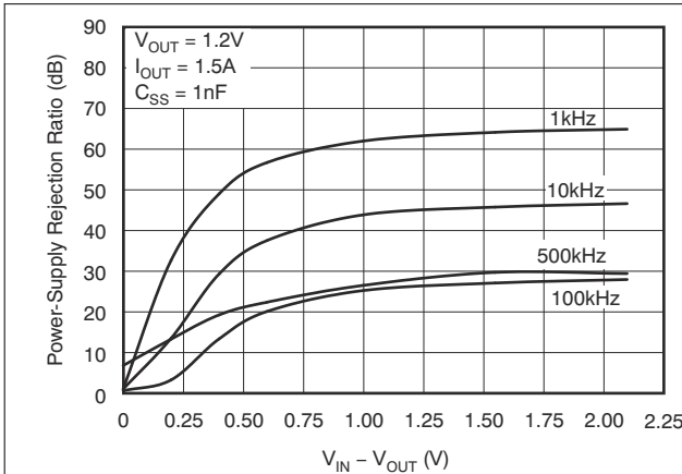
Figure 8-5. V_{IN} PSRR vs (V_{IN} - V_{OUT})
