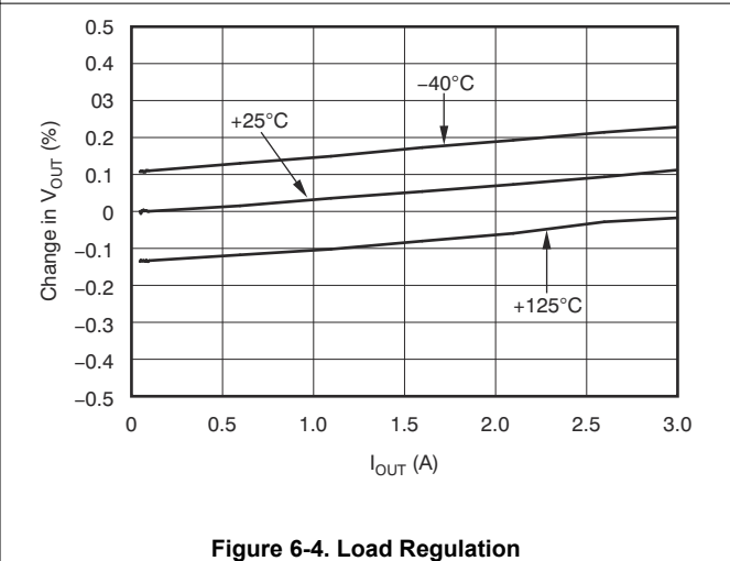
Figure 6-4. Load Regulation
