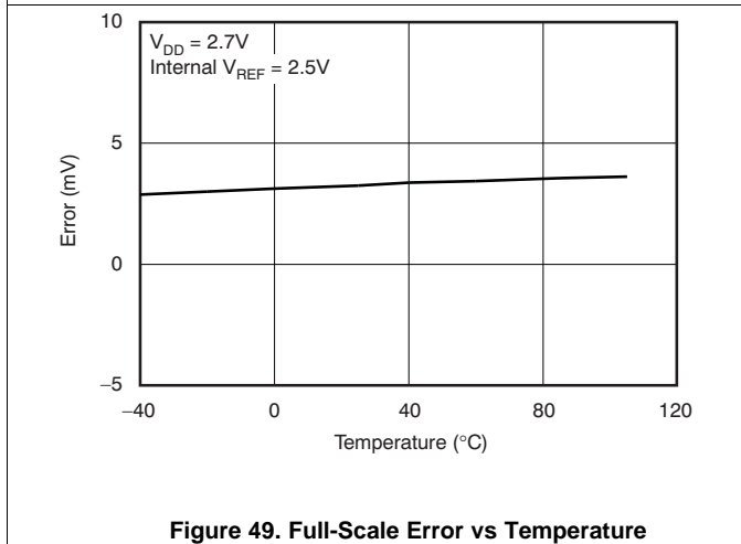
Figure 49. Full-Scale Error vs Temperature
