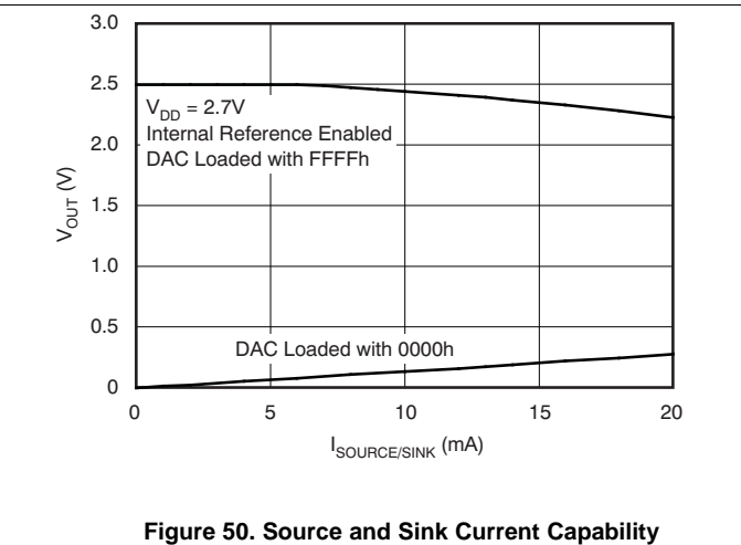
Figure 50. Source and Sink Current Capability
