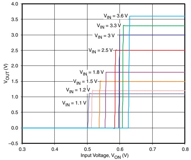
Figure 10. ON-Input Threshold
