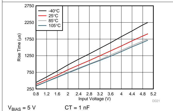
Figure 21. Rise Time vs Input Voltage ( V_{BIAS} = 5\text{ V} , CT = 1\text{ nF} )
