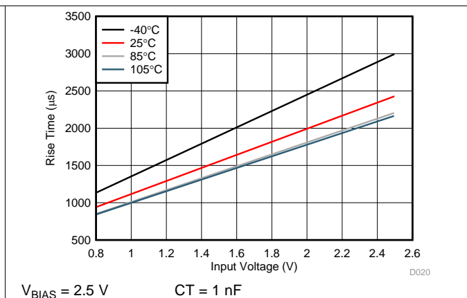
Figure 20. Rise Time vs Input Voltage
