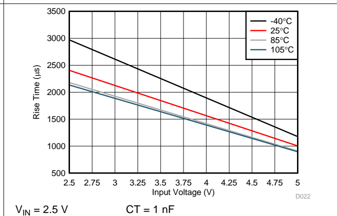
Figure 22. Rise Time vs Bias Voltage
