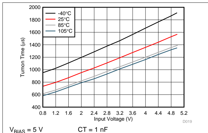
Figure 19. Turnon Time vs Input Voltage
