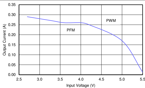
Figure 8-7. Regulation, AUTO Mode
