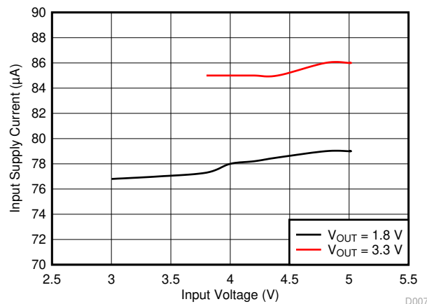
Figure 7-9. Typical No Load Input Supply Current
