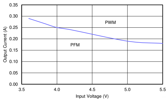
Figure 8-19. Regulation, AUTO Mode
