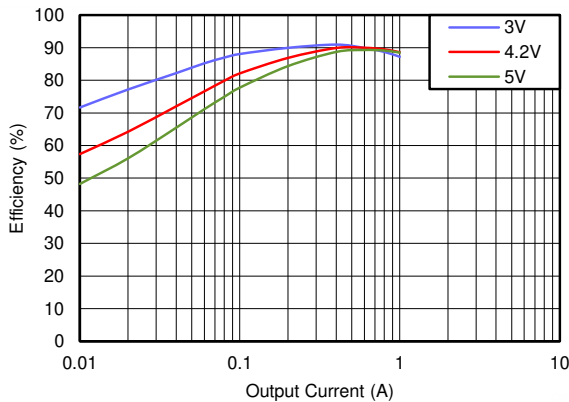
Figure 8-5. Efficiency
