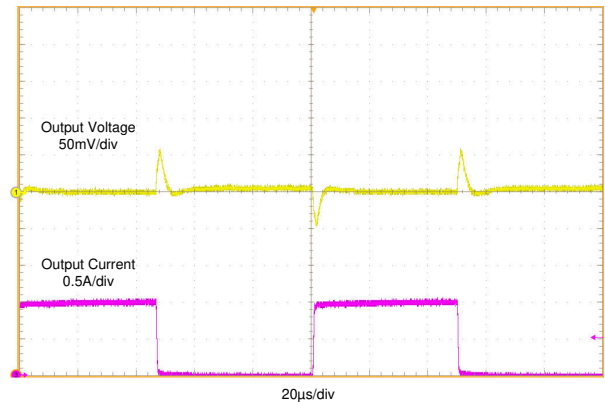
Figure 8-6. Load Transient In PWM
