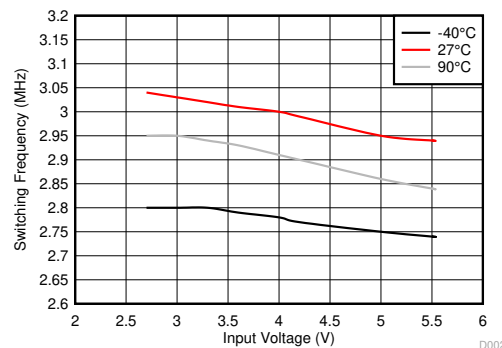
V_{IN} = 3.6\text{ V} I_{OUT} = 0\text{ A} PWM Mode
