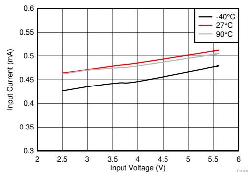
V_{FB} = 0.8\text{ V} PWM Mode
