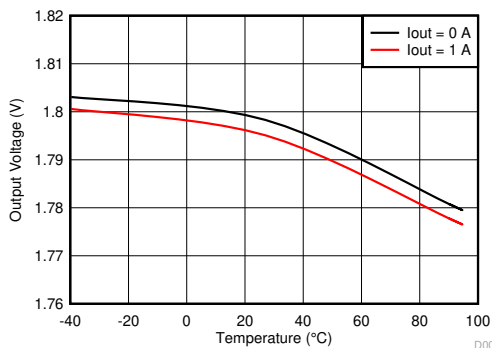
V_{IN} = 3.6\text{ V} PWM Mode V_{OUT} = 1.8\text{ V}
