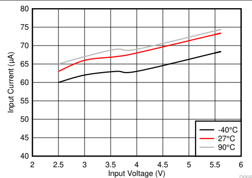
V_{FB} = 0.8\text{ V} AUTO Mode
