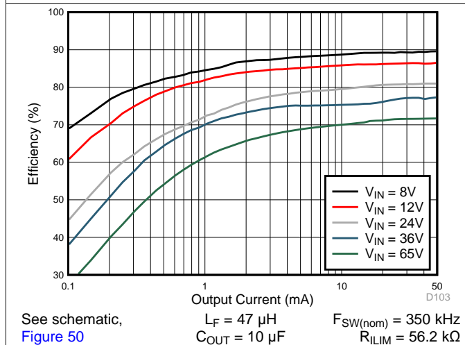
Figure 3. Converter Efficiency: 3.3 V, 50 mA, PFM
