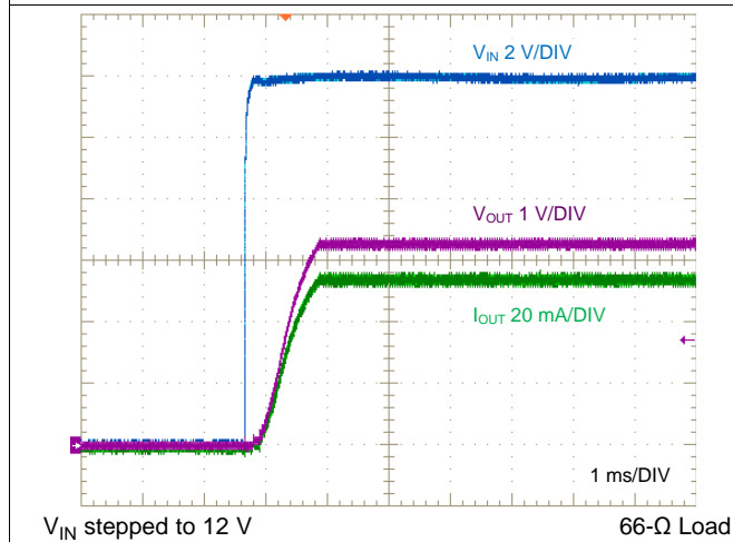
Figure 53. Startup, Full Load
