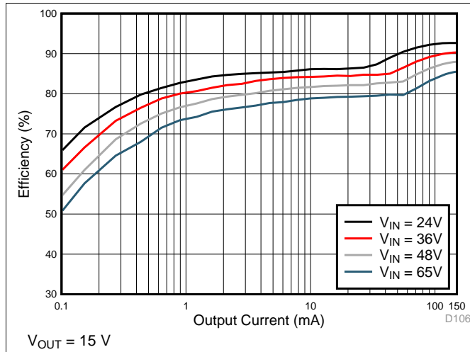
Figure 66. Efficiency
