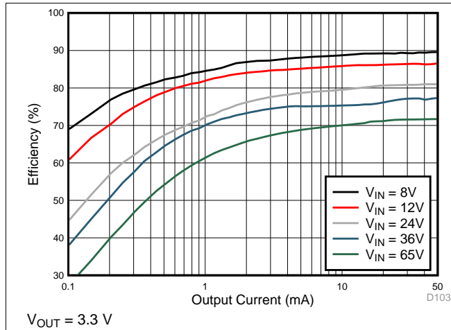
Figure 51. Efficiency
