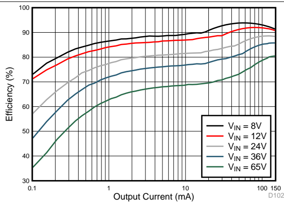
Figure 38. Efficiency
