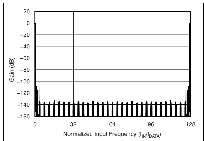
Figure 61. Frequency Response Out to f_{MOD} for High-Resolution Mode
