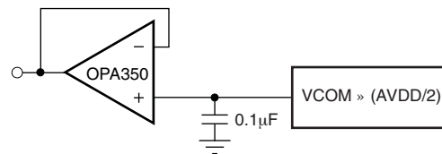
Figure 83. VCOM Output
