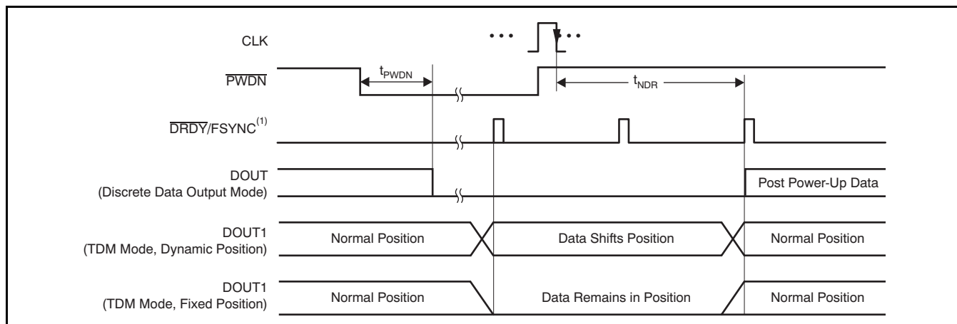
Figure 71. Power-Down Timing
