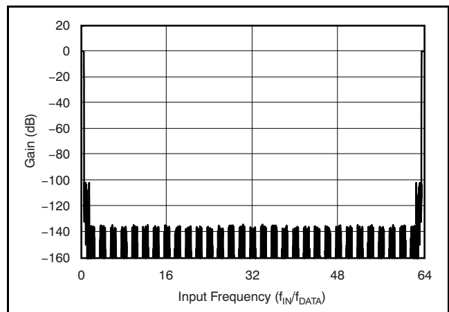
Figure 57. Frequency Response Out to f_{MOD} for High-Speed, Low-Power, and Low-Speed Modes
