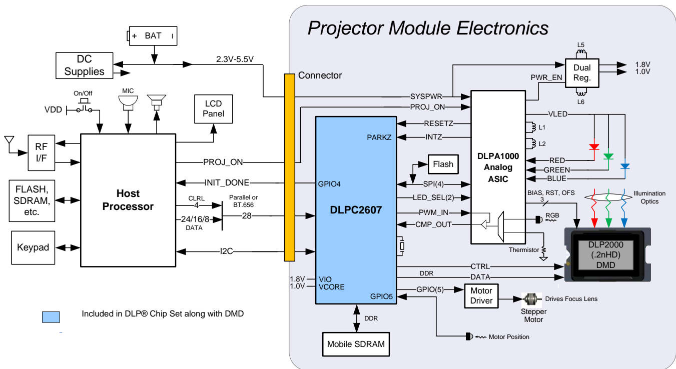
Figure 11. Block Diagram
