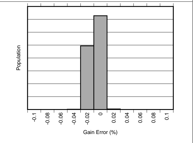
Figure 10. Gain Error Distribution (INA301A1)
