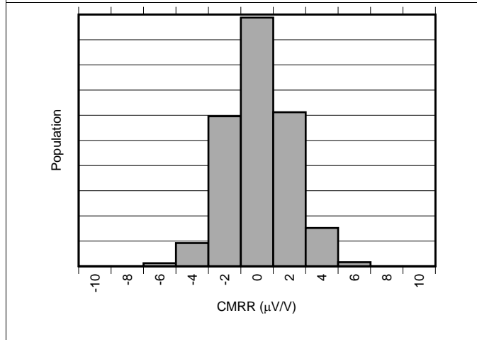
Figure 5. Common-Mode Rejection Ratio Distribution (INA301A1)
