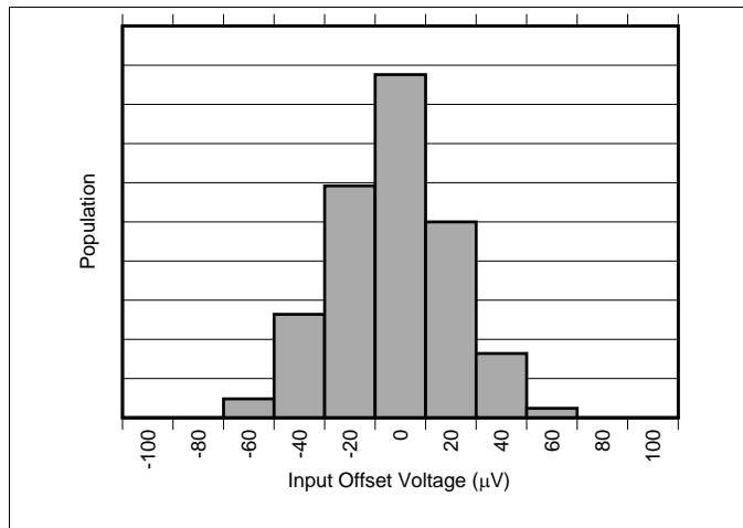
Figure 1. Input Offset Voltage Distribution (INA301A1)
