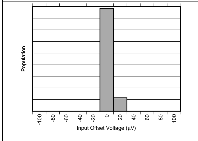
Figure 3. Input Offset Voltage Distribution (INA301A3)
