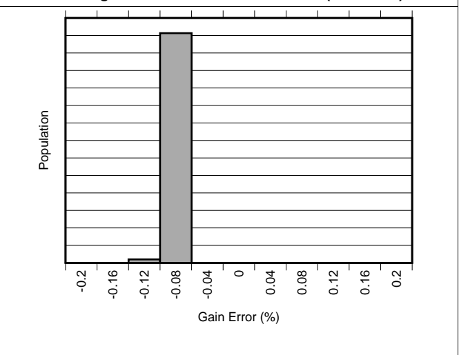
Figure 12. Gain Error Distribution (INA301A3)
