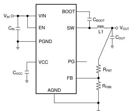
Figure 1. Simplified Schematic
