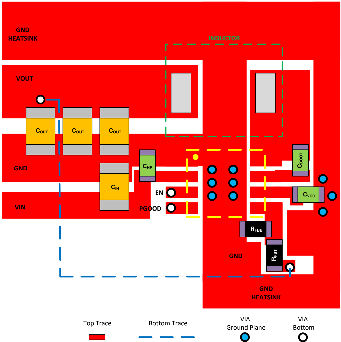
Figure 8. Example Layout
