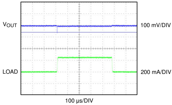
Figure 5-13. Load Transient
