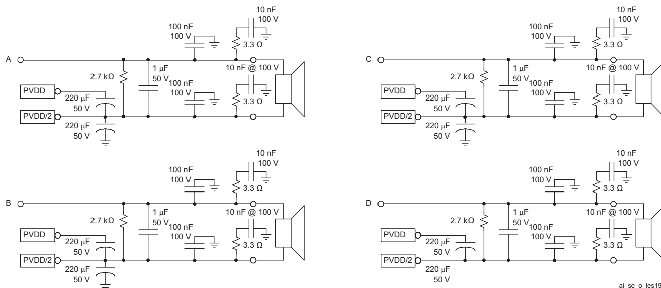
Figure 16. Typical SE Application (For Reference Only, component values and connection will change.)
