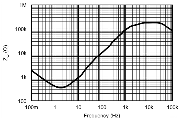
Figure 32. Open Loop Output Impedance
