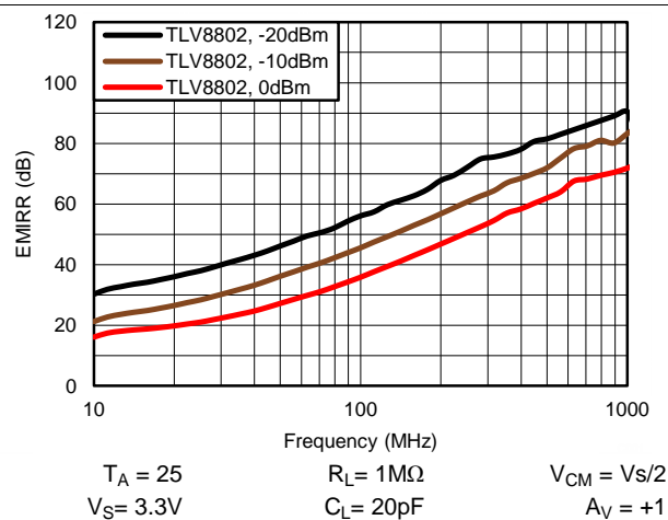
Figure 36. EMIRR Performance
