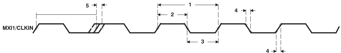
Figure 6-6. MXI1/CLKIN1 Timing
