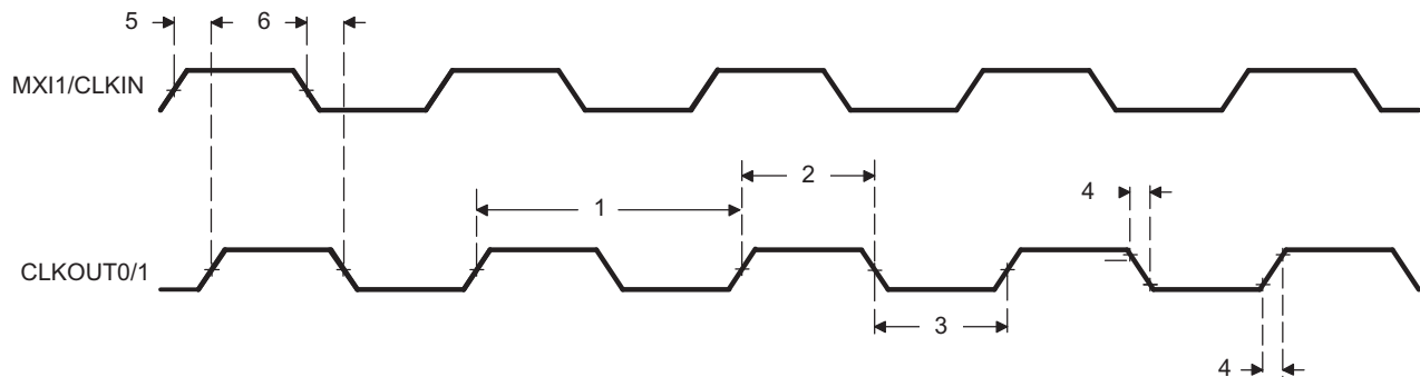
Figure 6-7. CLKOUT1 Timing
