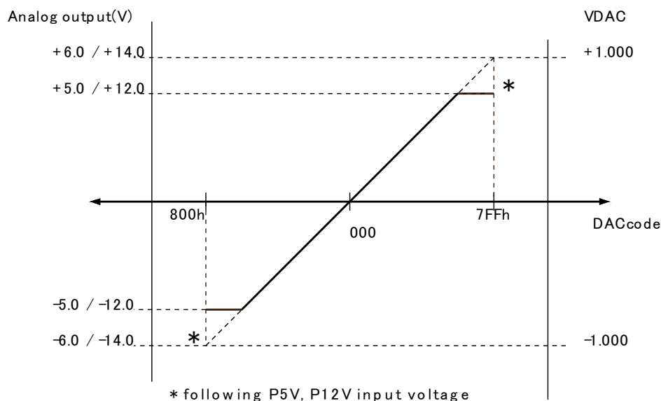
Figure 50. Output Voltage vs DAC Code
