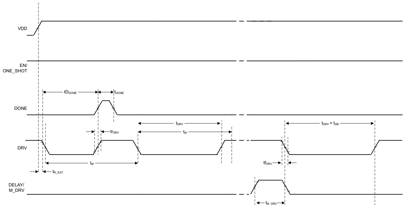
Figure 6-1. TPL5110-Q1 Timing
