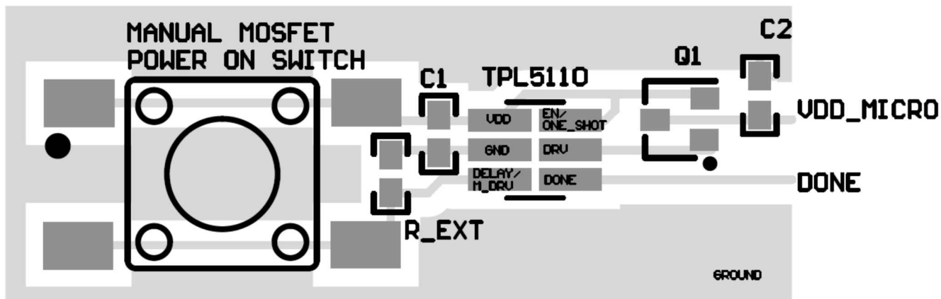
Figure 10-1. Layout
