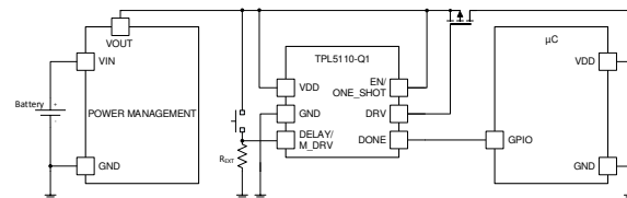
Simplified Application Schematic
