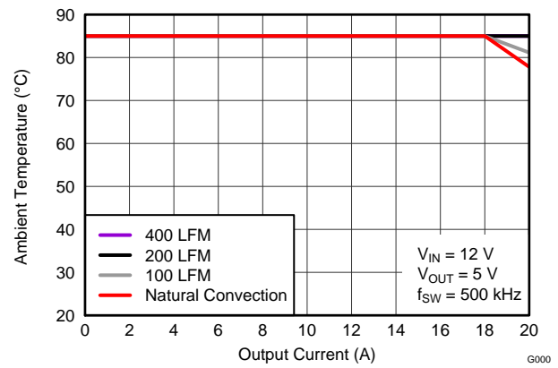
Figure 35. Safe Operating Area
