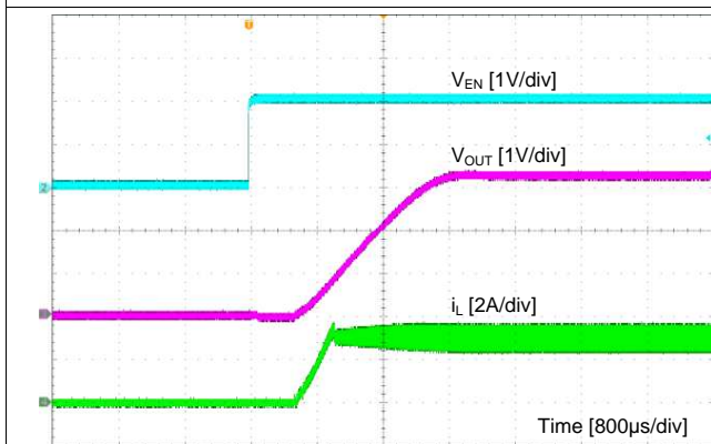
Figure 16. PSM Mode
