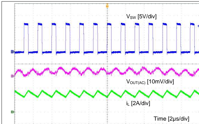
Figure 14. CCM Mode
