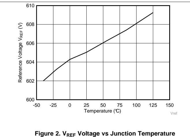
Figure 2. V_{REF} Voltage vs Junction Temperature
