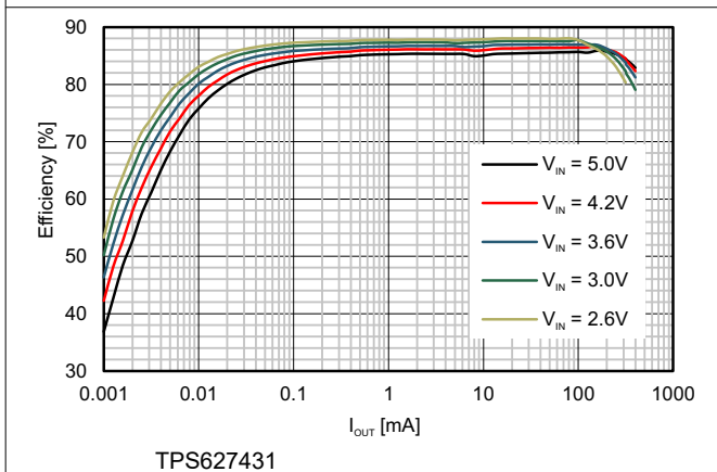
Figure 9-6. Efficiency vs Load Current; V_{OUT} = 1.4\text{ V}
