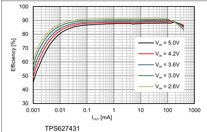
Figure 9-4. Efficiency vs Load Current; V_{OUT} = 1.9\text{ V}
