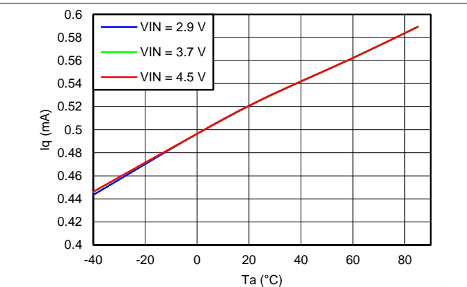
Figure 3. Quiescent Current
