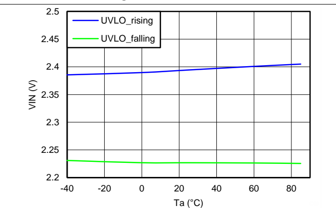
Figure 5. UVLO
