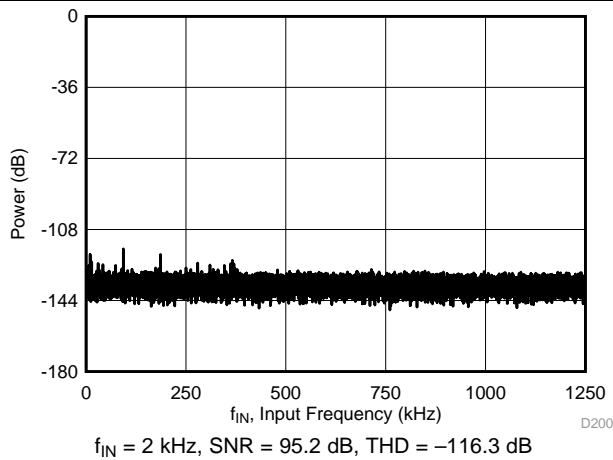
Figure 100. FFT with a 2-kHz Input Signal, Single-Ended Input
