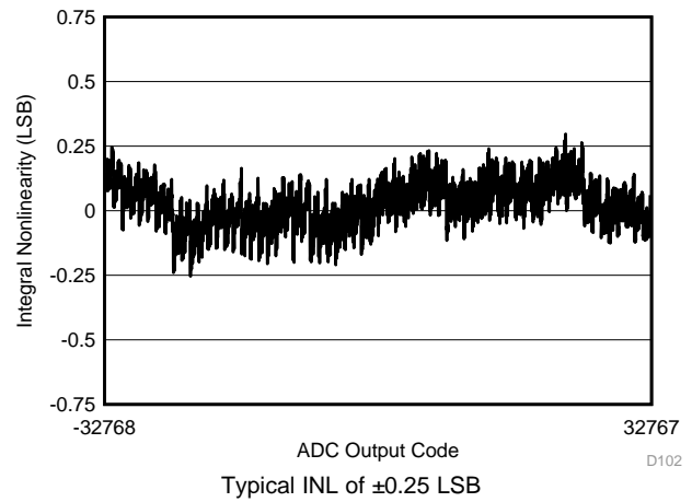
Figure 99. Typical INL, Differential Input
