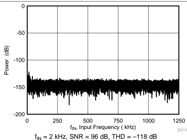
Figure 17. Typical FFT
