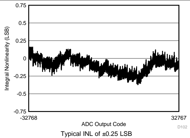
Figure 101. Typical INL, Single-Ended Input
