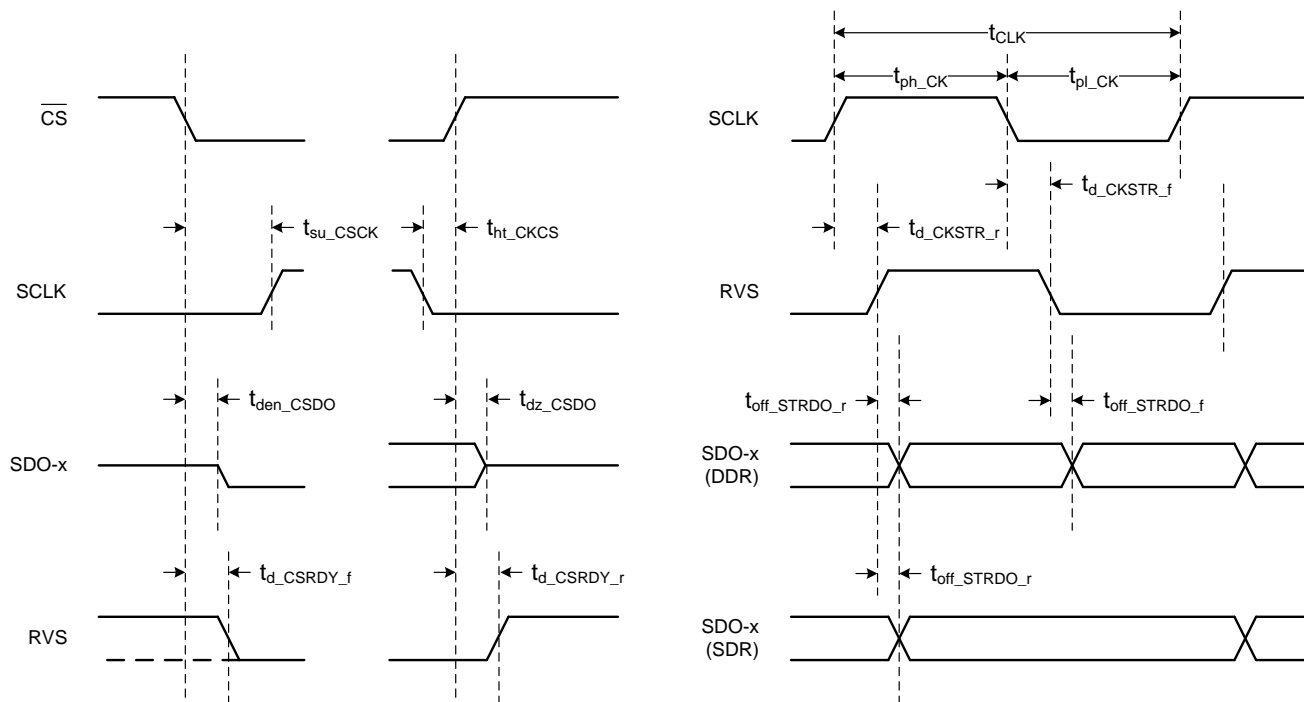
Figure 5. Source-Synchronous Serial Interface Timing Diagram (External Clock)
