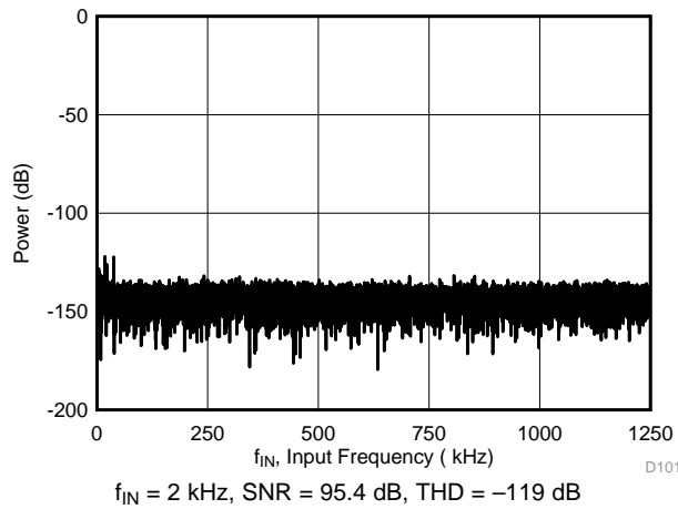
Figure 98. FFT with a 2-kHz Input Signal, Differential Input
