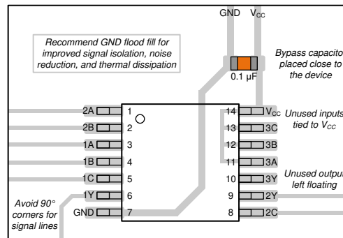
Figure 11-1. Example layout for the CD74HCT4075
