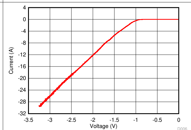
Figure 5-6. TLP I-V Curve, IO to GND Negative, t_p = 100ns
