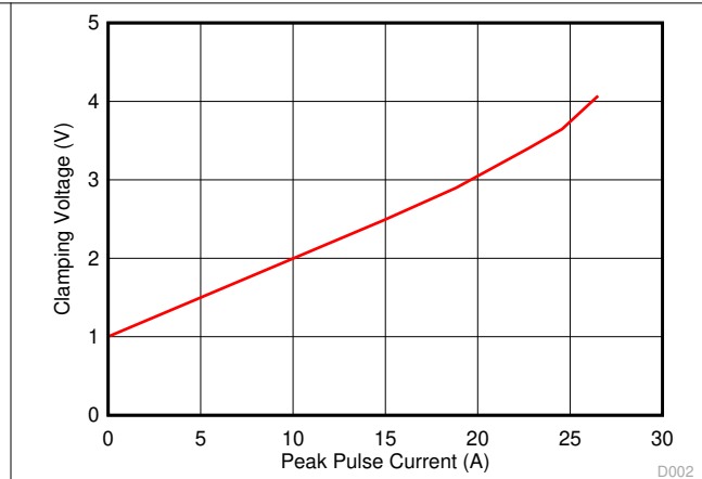
Figure 5-2. Clamping Voltage vs. Peak Pulse Current ( t_p = 8/20\mu s ), GND to Any IO Pin
