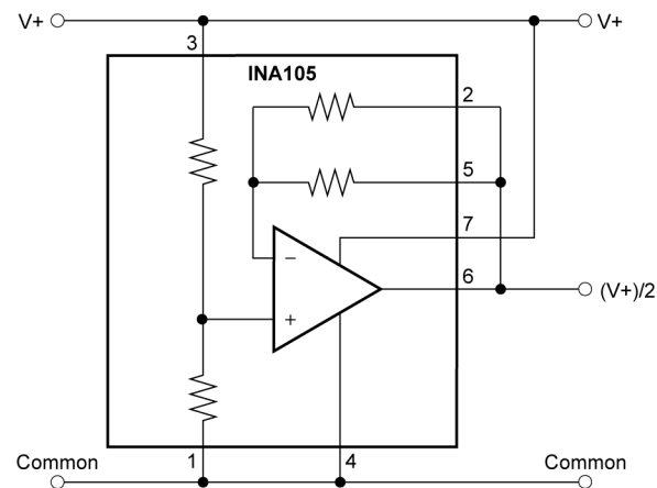
Figure 7-22. Pseudoground Generator
