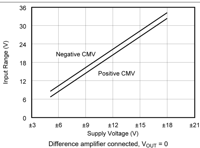
Figure 5-8. Common-Mode Input Range vs Supply
