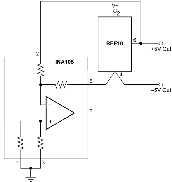
Figure 7-21. \pm 5\text{V} Precision Voltage Reference
