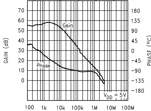
Open Loop Frequency Response, 5V
