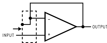
Figure 28. Typical Connections Of Guard Rings
