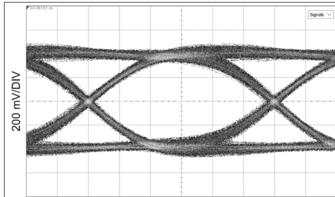
Measured at SDI_OUT1+ HOST_EQ0 = F, SDI_OUT2_SEL = L, OUT_CTRL = F Figure 24. 11.88 Gbps, TL = 20" FR4, Relocked
