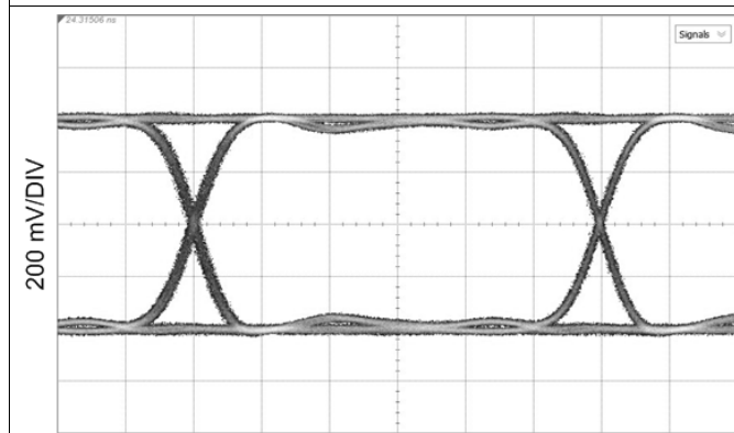
Measured at SDI_OUT1+ HOST_EQ0 = F, SDI_OUT2_SEL = L, OUT_CTRL = F Figure 28. 2.97 Gbps, TL = 20" FR4, Relocked
