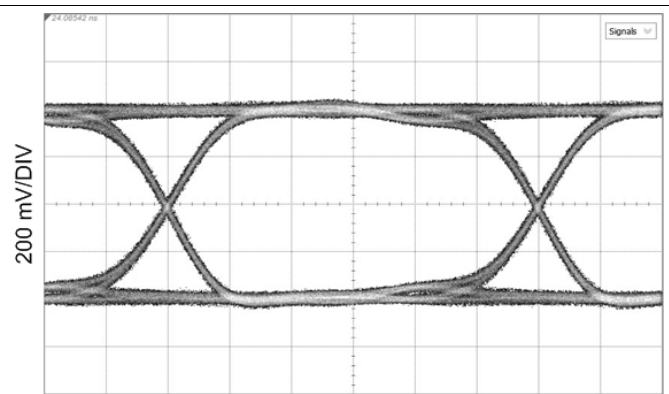
Measured at SDI_OUT2+ HOST_EQ0 = F, SDI_OUT2_SEL = L, OUT_CTRL = F Figure 27. 5.94 Gbps, TL = 20" FR4, Relocked
