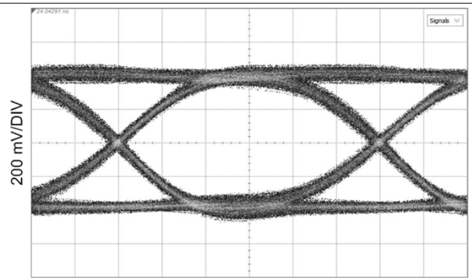
Measured at SDI_OUT2+ HOST_EQ0 = F, SDI_OUT2_SEL = L, OUT_CTRL = F Figure 25. 11.88 Gbps, TL = 20" FR4, Relocked
