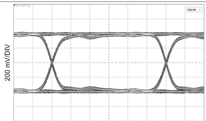
Measured at SDI_OUT2+ HOST_EQ0 = F, SDI_OUT2_SEL = L, OUT_CTRL = F Figure 29. 2.97 Gbps, TL = 20" FR4, Relocked
