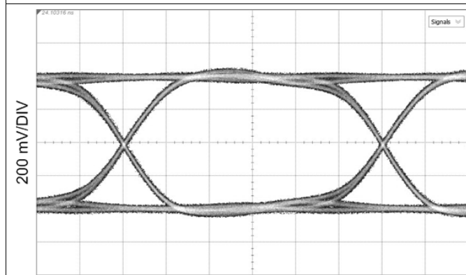
Measured at SDI_OUT1+ HOST_EQ0 = F, SDI_OUT2_SEL = L, OUT_CTRL = F Figure 26. 5.94 Gbps, TL = 20" FR4, Relocked
