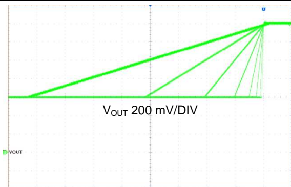
Figure 46. Start-up with NRST, Forced PWM
