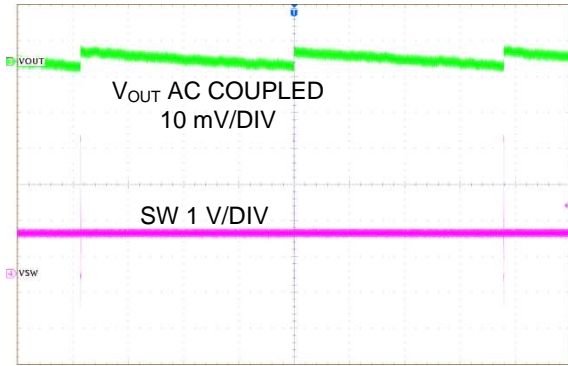
Figure 43. Output Voltage Ripple, PFM Mode
