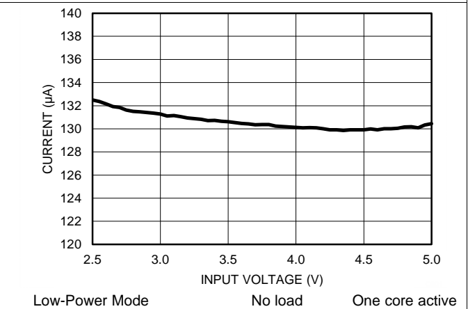
Figure 5. Low-Power PFM Mode Current Consumption vs V_{IN}
