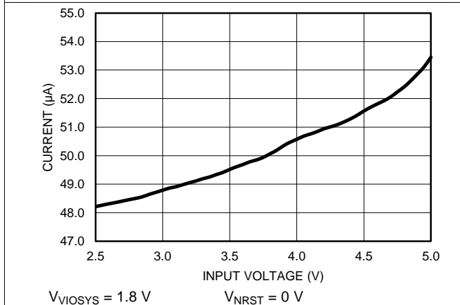
Figure 4. Standby Mode Current Consumption vs V_{IN}
