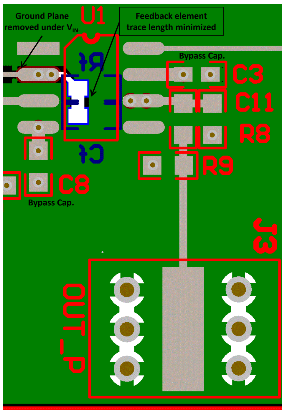
Figure 38. Layout Recommendation
