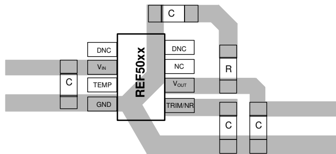
Figure 12-1. Layout Example
