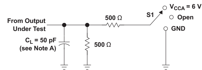
LOAD CIRCUIT
