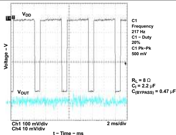
Figure 9. GSM Power Supply Rejection vs Time
