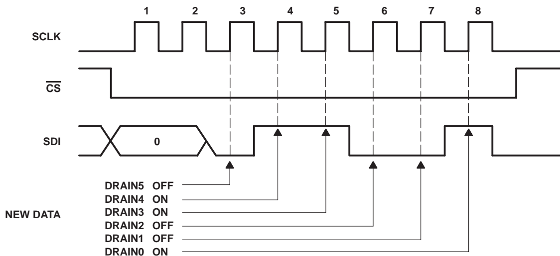
Figure 2. Serial Input Control
