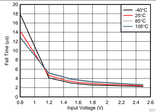
Figure 14. Fall Time vs Input Voltage
