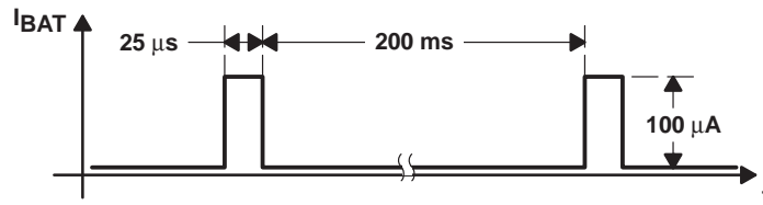
Figure 1. BATTOK Timing
