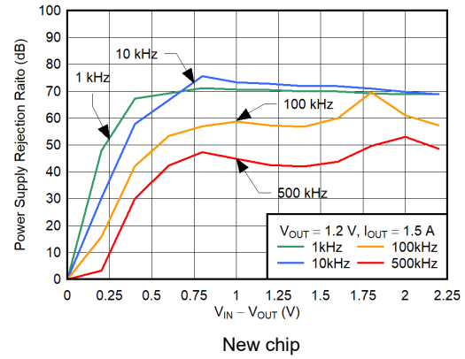
Figure 5-20. V IN PSRR vs (V IN - V OUT )
