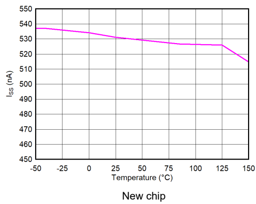
Figure 5-28. Soft-Start Charging Current (I SS ) vs Temperature (T J )
