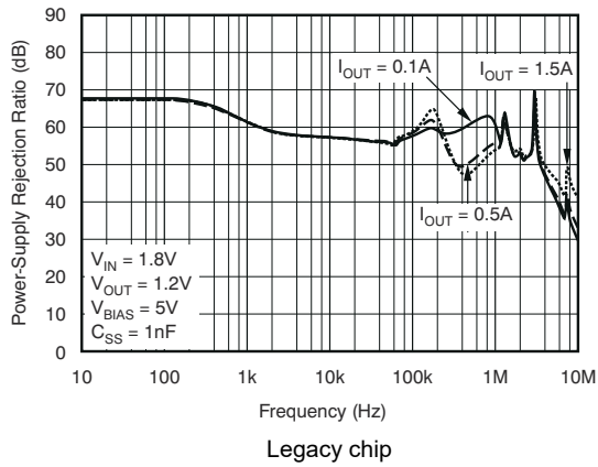
Figure 5-15. V_{BIAS} PSRR vs Frequency Legacy chip
