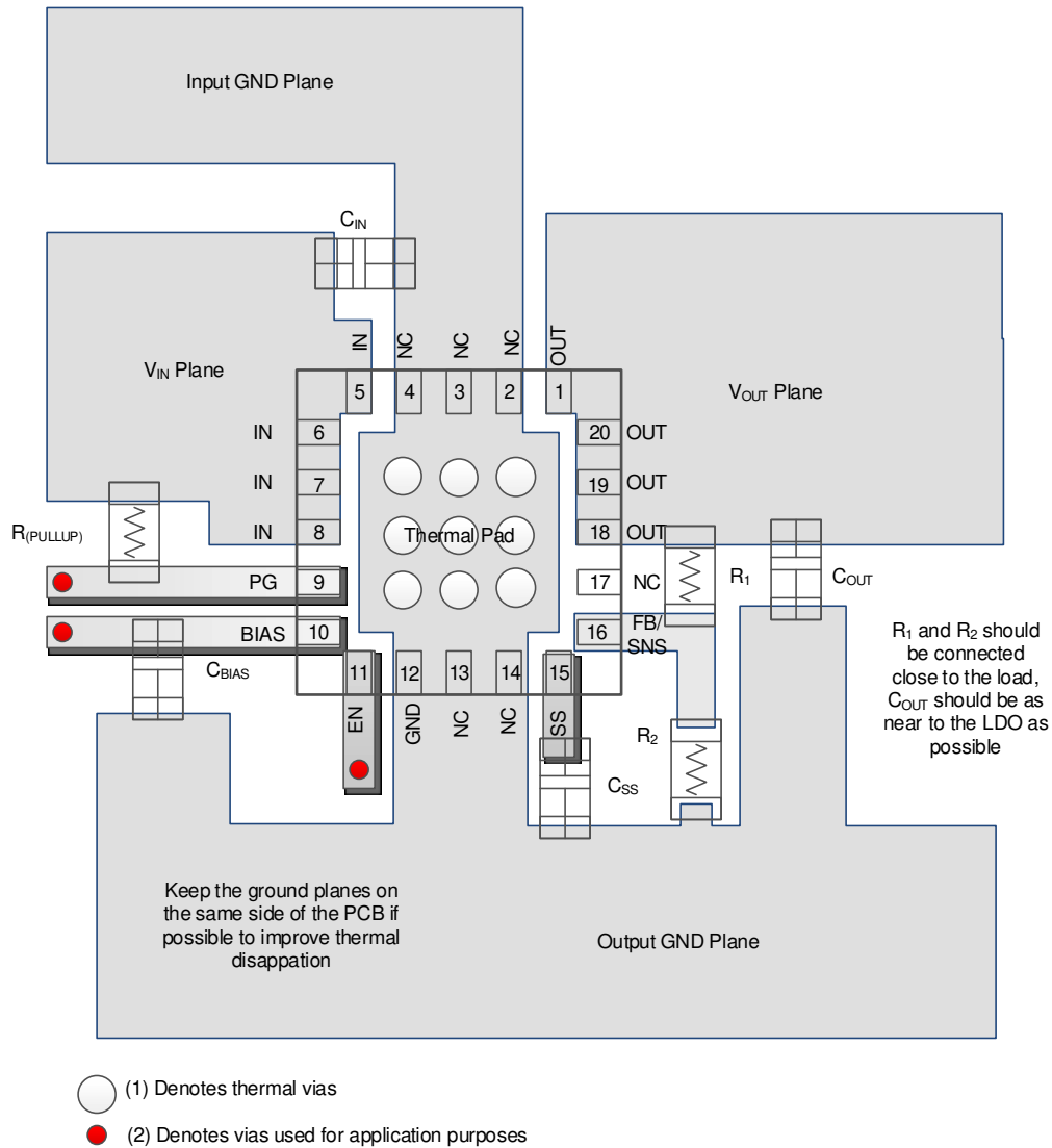
Figure 7-16. Layout Example (RGW Package)
