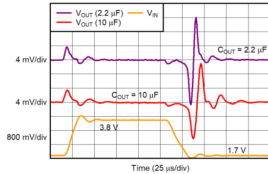
Figure 7-4. V_{IN} Line Transient
