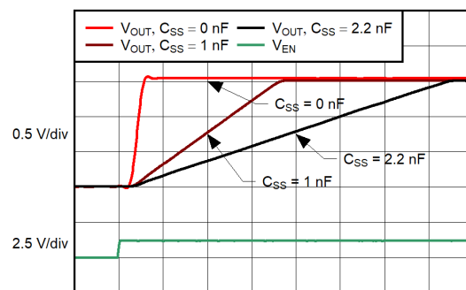
Turn-On Response
