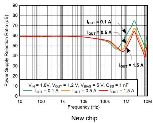
Figure 5-16. V_{BIAS} PSRR vs Frequency New chip
