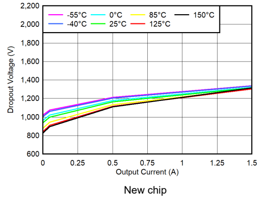
Figure 5-14. V_{BIAS} Dropout Voltage vs I_{OUT} and Temperature ( T_J ) New chip
