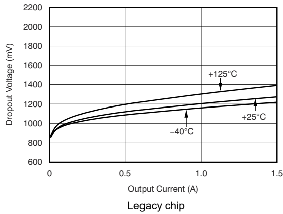
Figure 5-13. V_{BIAS} Dropout Voltage vs I_{OUT} and Temperature ( T_J ) Legacy chip
