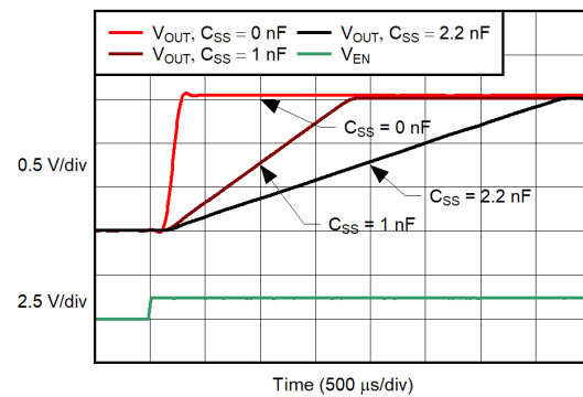
Figure 7-6. Turn-On Response
