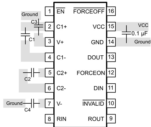
Figure 10-1. Layout Diagram
