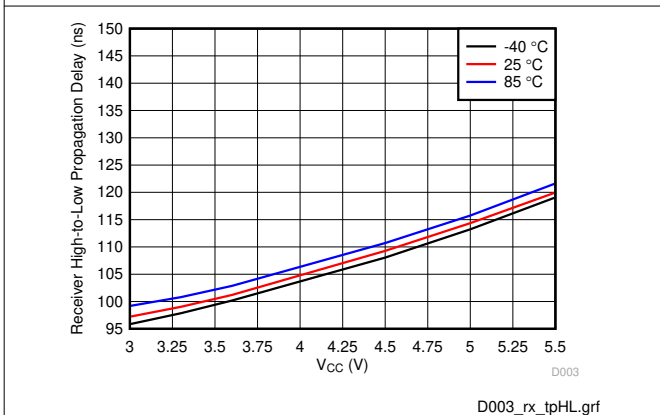
Figure 6-3. Receiver Path High-to-Low Propagation Delay vs T_A and Supply Voltage (RGT Package)
