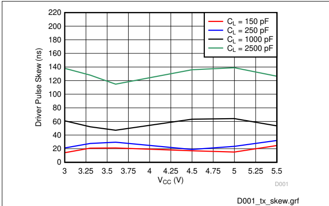
Figure 6-1. Driver Pulse Skew vs Load Capacitance and Supply Voltage at T_A = 25\text{ }^\circ\text{C} (RGT Package)
