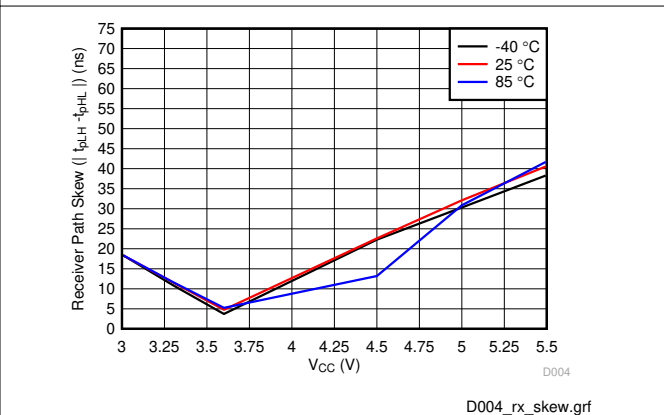
Figure 6-4. Receiver Pulse Skew ( t_{pLH} - t_{pHL} ) vs T_A and Supply Voltage (RGT Package)
