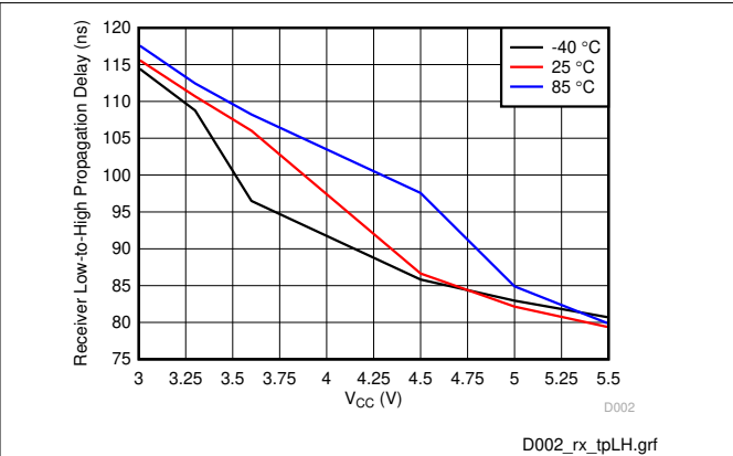
Figure 6-2. Receiver Path Low-to-High Propagation Delay vs T_A and Supply Voltage (RGT Package)
