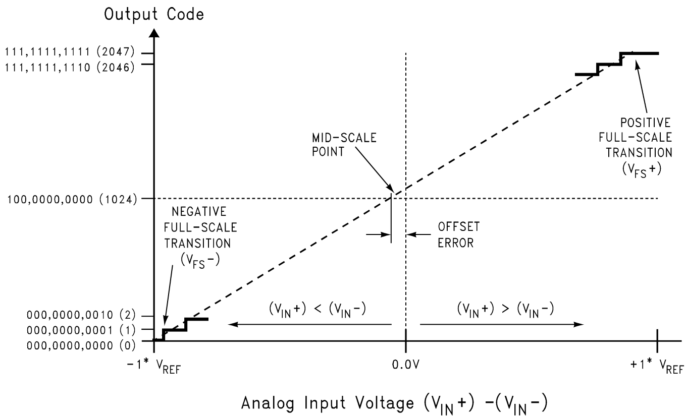
Figure 2. Transfer Characteristic (Offset Binary Format)
