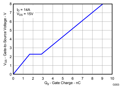
GATE CHARGE
