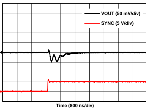
Figure 62. VOUT Full-Scale Settling Time, Rising Edge
